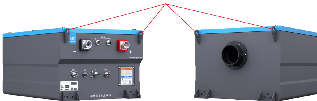
Figure 2 - RS battery module lifting points
